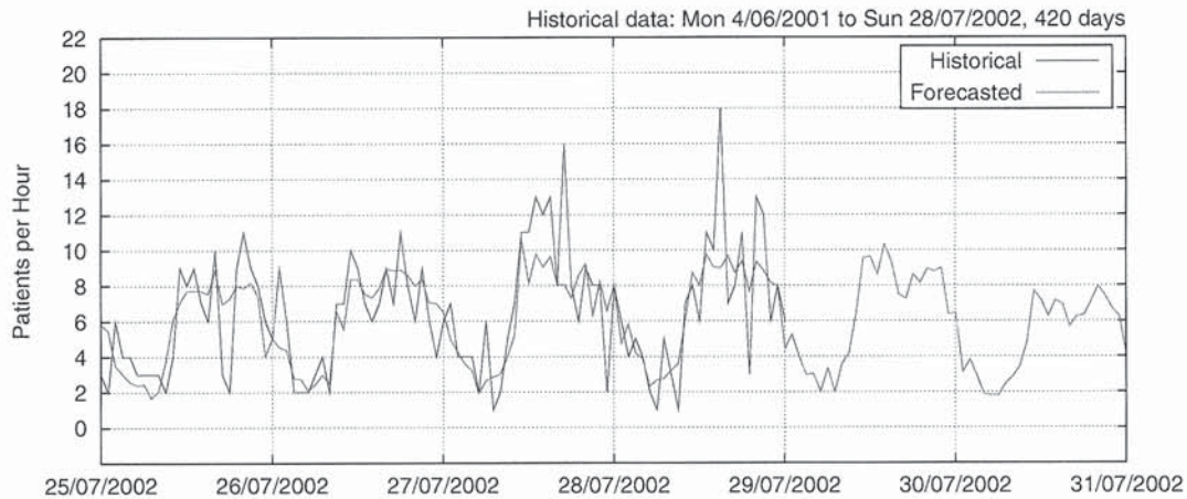
Figure 2: Hourly historical and forecasted data 25/7/2002–31/7/2002
