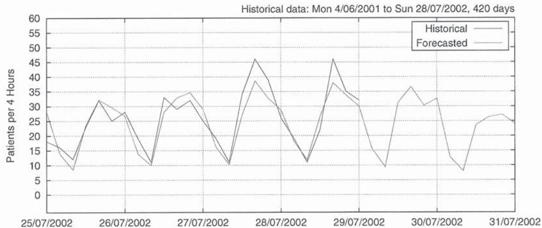
Figure 3: Four-hourly historical and forecasted data 25/7/2002–31/7/2002
